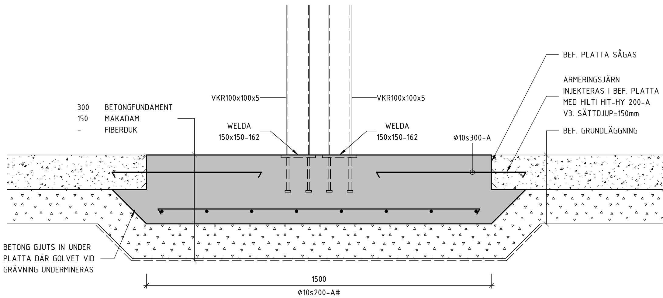
C001 1 : 10
